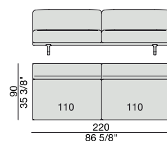
CENTRAL UNIT 220x90
