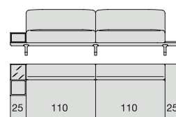
SOFA/CENTRAL UNIT with Coffee table and Container 220x90
