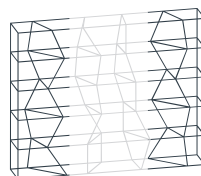
cod. 16.17 Moduli laterali | Side modular element cm L 125 x P 38 x H 182 inch L 49.2 x W 15 x H 72
