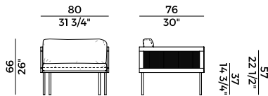
880/PR-OUT lounge \ lounge armchair
