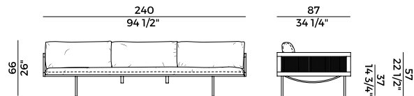
880/DR-OUT divano \ sofa
