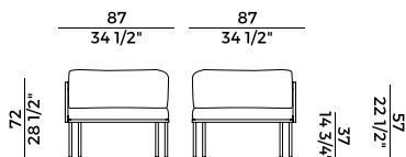
880/DR-200-OUT divano \ sofa
