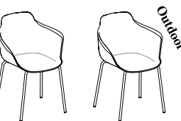
cod. 34.19 MOOD cm L61 x P57 x H81/46 inch L24 x W22.4 x H31.9/18.1
