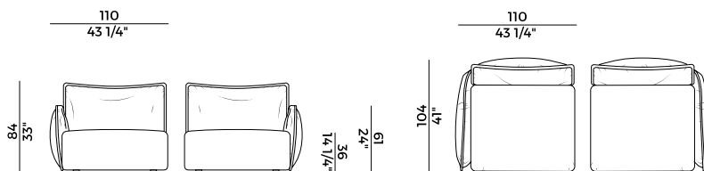
935/DT modulo laterale destro e sinistro \ right and left side unit
